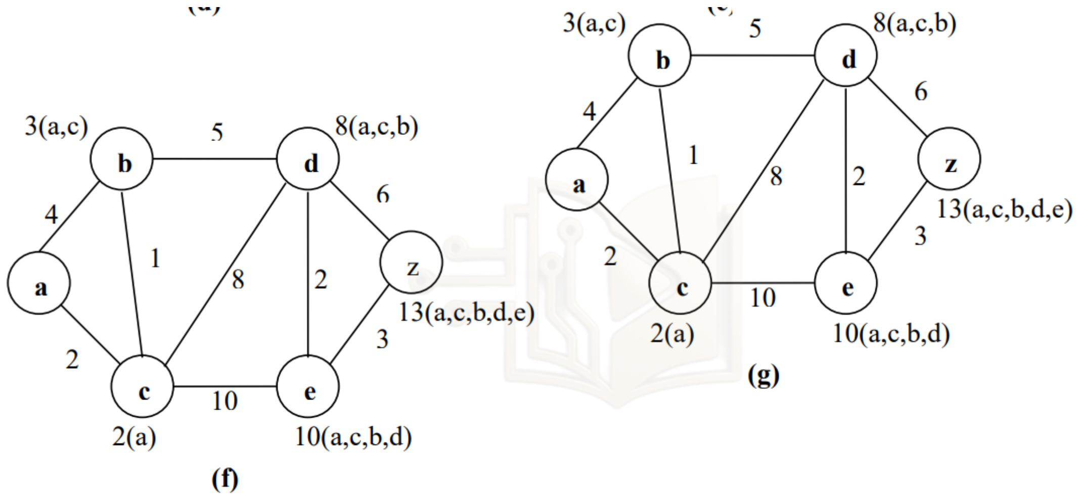
Fig: Using Dijkstra's Algorithm to find shortest path from a to z
